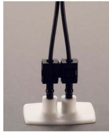
Figure 11. Duplex Polishing Disc
